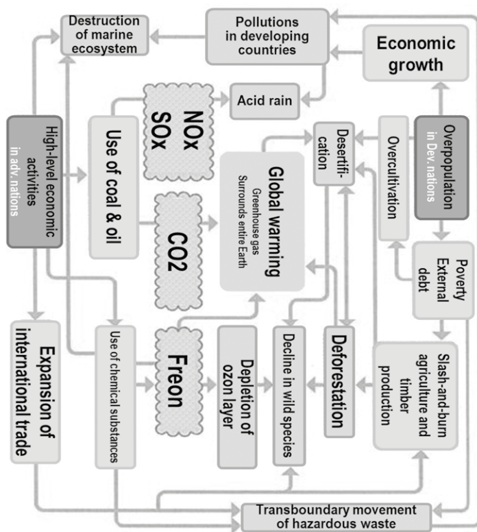
Fig. 2: Diagram of the complex mechanism of environmental issues (Kyoiku Shuppan (Nakamura, T. et al.), 2015, p. 204) (transl. and mod. by author; same applied to the following figures)
