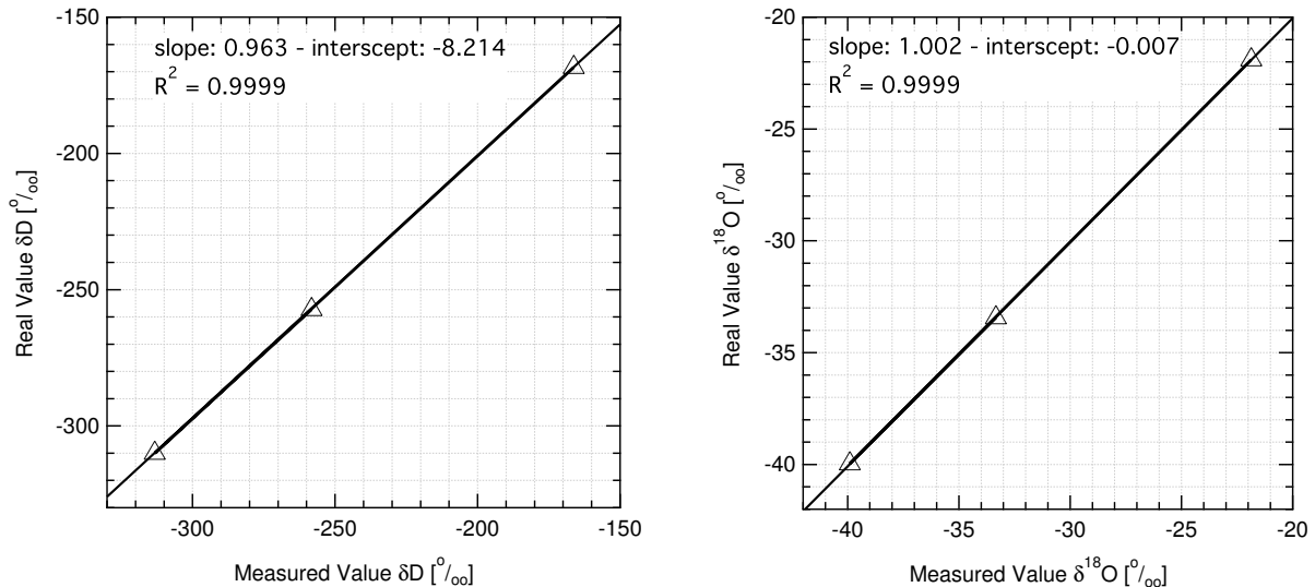
Fig. 3. VSMOW calibrations with three water standards “–22”, “–40” and “NEEM”; Left – \delta\text{D} , right – \delta^{18}\text{O} .
