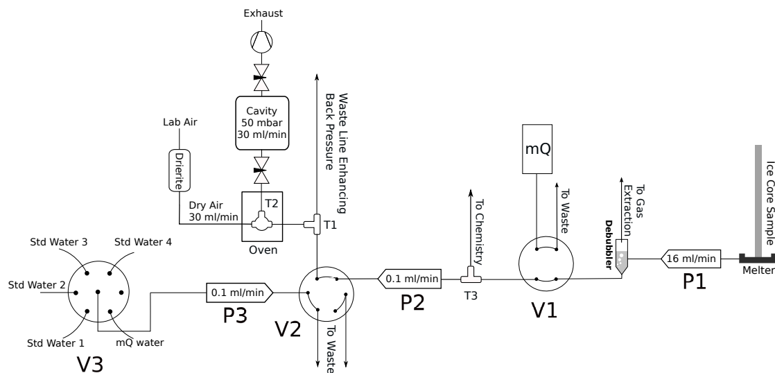
Fig. 1. Block diagram of the CFA-CRDS system.
