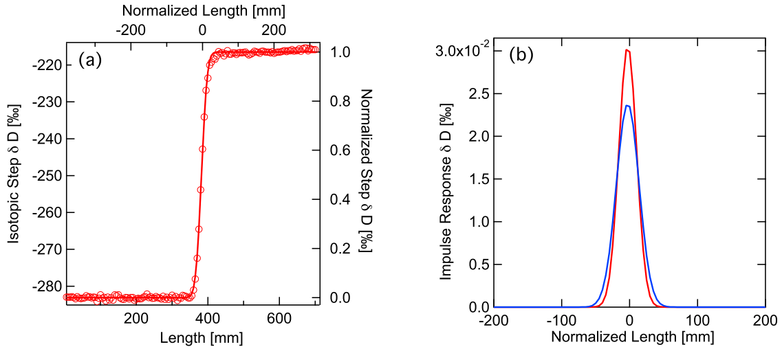
Fig. 7. (a) Isotopic \delta D step. The length scale is normalized so normalized length = 0 when the normalized \delta D value equals 0.5 ‰. (b) Impulse Response of the system for \delta D based on the step response (red) and the spectral analysis (blue) with \sigma_{cfa} = 13.4 and 16.4 mm, respectively.
