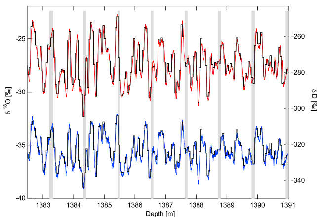
Fig. 6. Comparison CRDS-CFA with 5 cm discrete samples for \delta D (top) and \delta^{18}O (bottom). Bars indicate the position and width of sections with missing/removed data.
