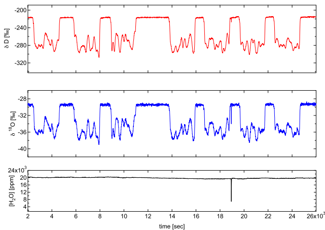
Fig. 2. Raw signals spanning 7 CFA runs on 29 May 2010.
