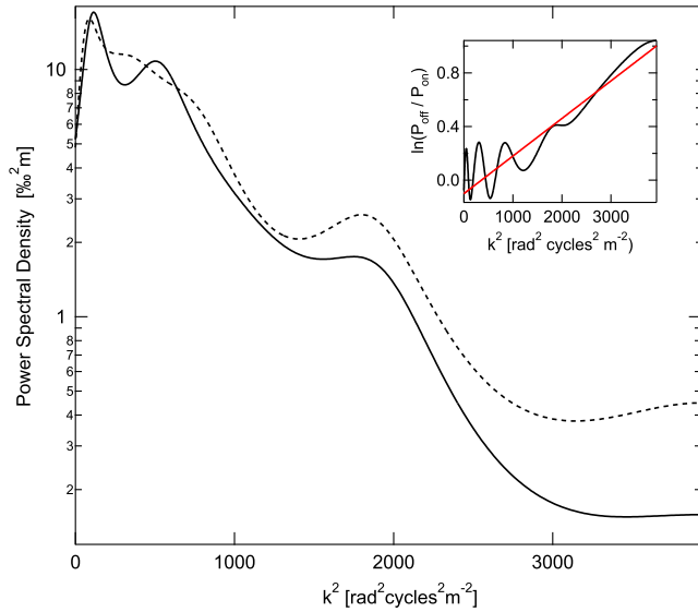
Fig. 9. Calculation of the diffusion length for the transfer function of the CFA system. The dashed and solid lines represent, respectively the power spectral density of the offline discrete data and the CFA data averaged on a 5 cm resolution.
