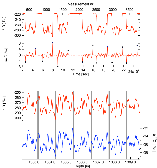
Fig. 4. The beginning and end of each CFA run is determined by the extrema of the 1st derivative of the isotopic signal, presented on the top graph. With gray bars we indicate the position and width of sections with data that are missing due to breaks in the ice, or removed in order to account for the transition from mQ water to sample and vice versa.
