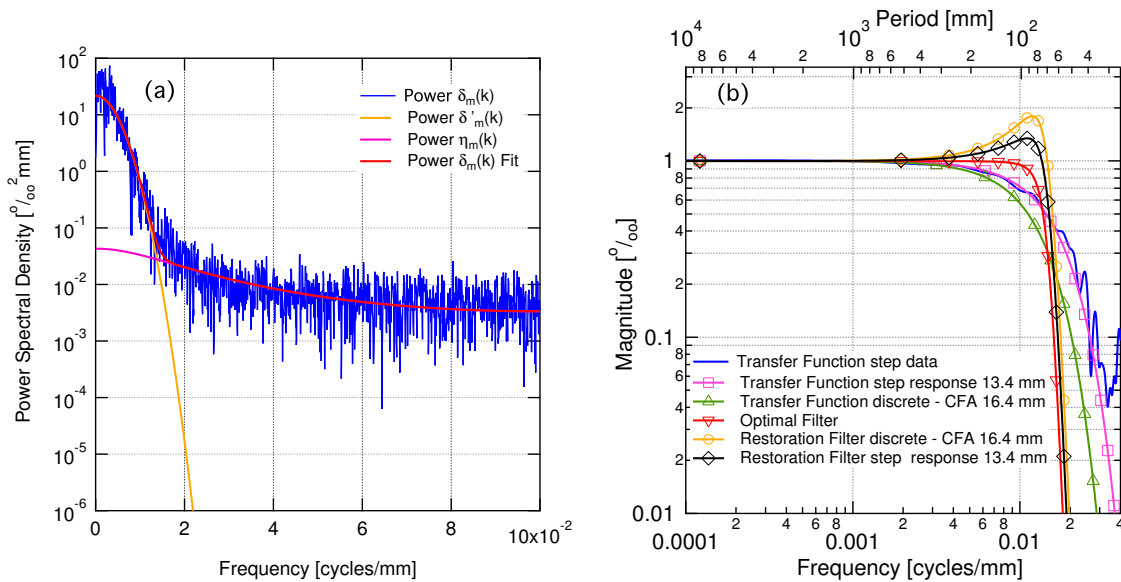
Fig. 8. (a) Power spectral density of \delta D . (b) Transfer function calculated based on the step response with \sigma_{cfa} = 13.4 mm (pink – squares) and the comparison between discrete and CFA analysis with \sigma_{cfa} = 16.4 mm (green – triangles). Restoration filters built considering the two different transfer functions are illustrated with orange circles ( \sigma_{cfa} = 16.4 mm) and black diamonds ( \sigma_{cfa} = 13.4 mm).
