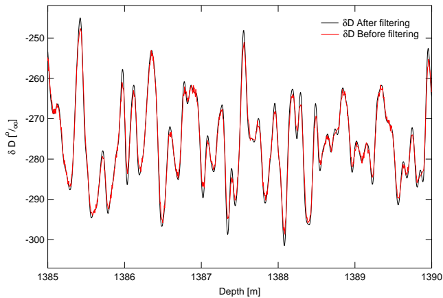
Fig. 10. \delta D signal before and after optimal filtering.
