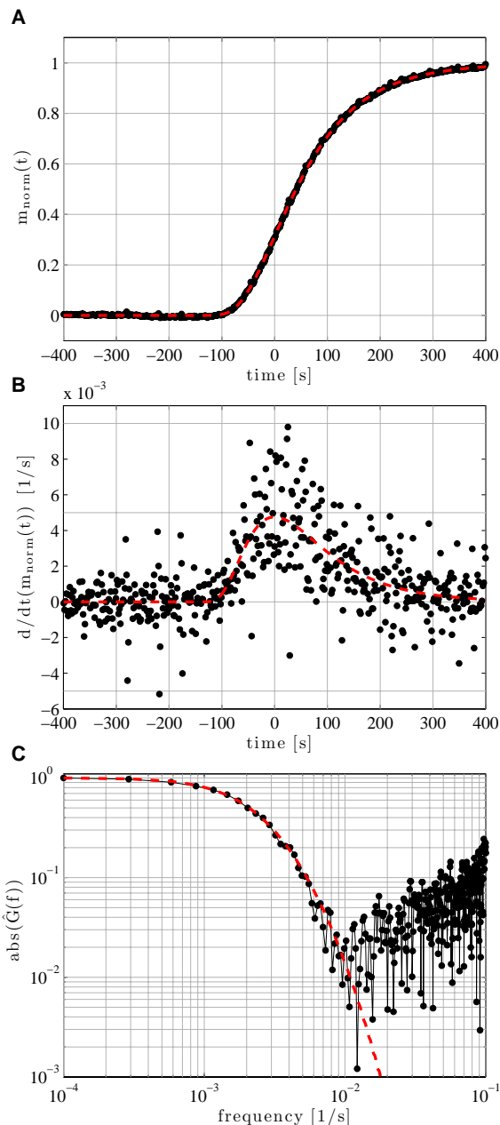
Fig. 5. (A) Normalized response of the complete experimental setup (except melt head) to a stepwise change in CH 4 mixing ratio (black dots) and a cdf fit (dashed red line) as a function of measurement time. (B) The derivative of the normalized step response (black dots) and of the cdf fit (dashed red line) with respect to the measurement time. (C) The transfer functions of the experimental setup (black dots) and of the theoretical case of zero-noise measurements (dashed red line).
