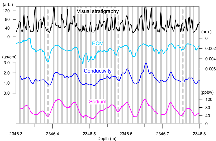
Fig. 2. Example of annual layer counting within the stadal preceding GI-14. Same legend as for Fig. 1. The counting of this section is mostly based on visual stratigraphy and ECM profiles which have the highest resolution.
