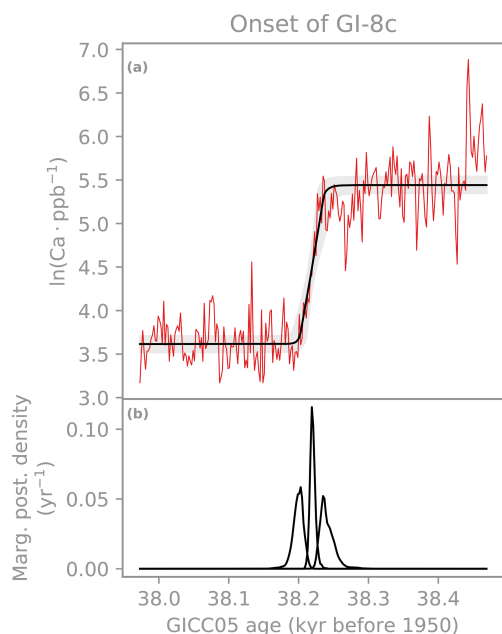
Figure 2. Example of a fitted ramp for the \text{Ca}^{2+} data from the onset of GI-8c. Panel (a) shows the data together with the marginal posterior median of the fitted ramp (thick black line). Shaded areas indicate the marginal posterior 5th and 95th percentiles. Panel (b) shows the marginal posterior densities for the onset, midpoint and endpoint of the transition (from right to left).
