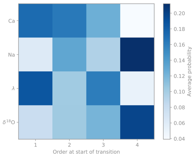
Figure 5. Combined order statistics for the onset of the transition. The colours indicate the probability of observing the onset of the transition in the parameter on the y axis at the position on the x axis. This illustrates that during the onset of the DO warming, the changes in accumulation and \text{Ca}^{2+} concentrations about equally likely occur first, whereas the transitions in \text{Na}^+ and \delta^{18}\text{O} about equally likely occur last.
