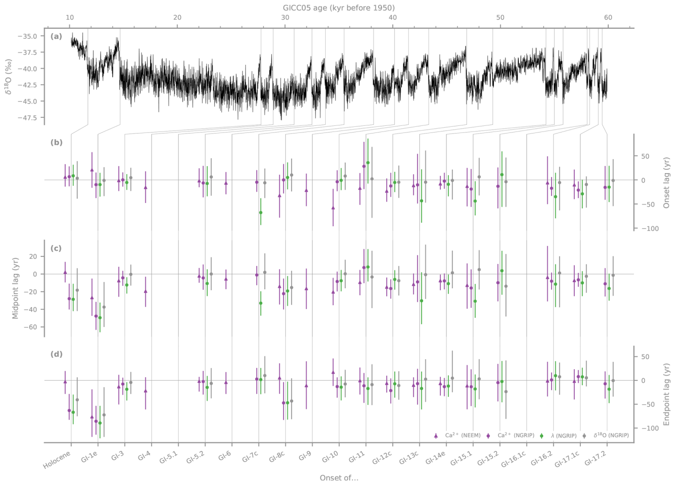
Figure 3. Timing differences for the individual interstadial onsets: (a) the NGRIP \delta^{18}\text{O} record, (b–d) timing difference of NGRIP \text{Ca}^{2+} , layer thickness ( \lambda ) and \delta^{18}\text{O} records, as well as the NEEM \text{Ca}^{2+} record relative to the transition in the respective \text{Na}^+ records at the onset (b), midpoint (c) and end (d) of the transition. No timing results are given for transitions where there are data gaps in one of the necessary datasets. Error bars show the marginal posterior 5th and 95th percentiles and the symbol the marginal posterior median. Note the different axis scaling for the start, midpoints and endpoints. All inferred absolute timings, the transition durations and the lags relative to \text{Na}^+ can be found in the Supplement.
