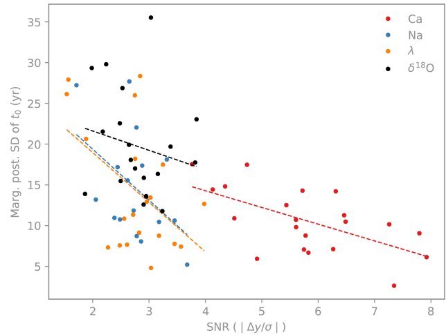
Figure A1. Timing uncertainty as a function of SNR for the NGRIP datasets. The uncertainty in the onset of the transition increases with lower SNR, as defined by the amplitude of the transition over the amplitude of the noise. Note that the linear fits are only for illustration.
