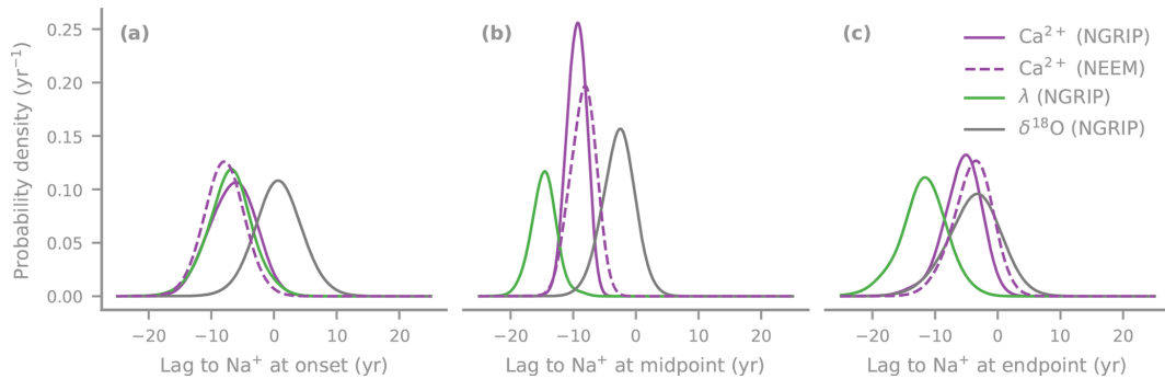
Figure 4. Combined probability density estimates of the lag of the \text{Ca}^{2+} , layer thickness and \delta^{18}\text{O} transitions relative to the respective point in the \text{Na}^+ records for the onset (a), midpoint (b) and end (c) of all transitions from stadial to interstadial for the two cores.
