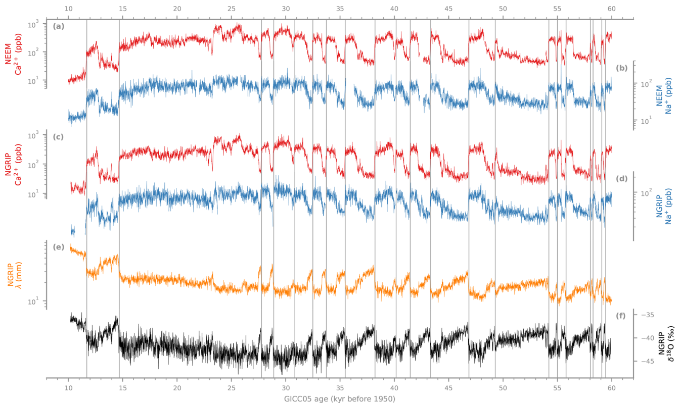
Figure 1. Investigated records from the NEEM (a, b) and NGRIP ice cores (c–f). Panels (a), (d) show the new aerosol records of \text{Ca}^{2+} (a, c) and \text{Na}^+ (b, d) alongside the NGRIP layer thickness ( \lambda ) (e) and ice \delta^{18}\text{O} records (f). All records are shown as decadal averages on their respective version of the GICC05 age scale relative to 1950 (Svensson et al., 2008; Rasmussen et al., 2013). The vertical lines mark the investigated interstadial onsets as given by Rasmussen et al. (2014). Note that the vertical scales for the aerosols and annual layer thickness are logarithmic.
